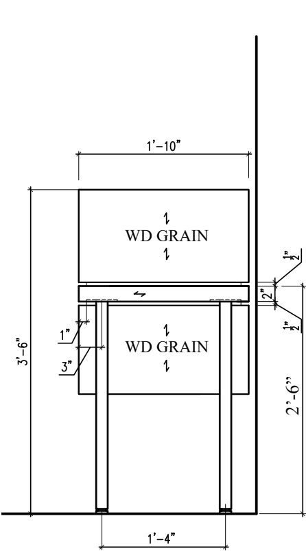
SIDE ELEVATION
